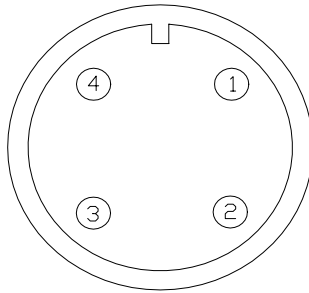
Front View (face)
